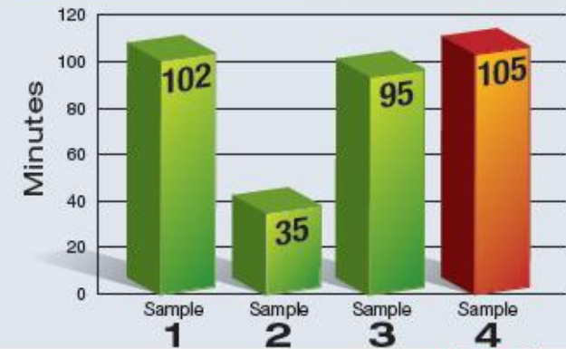
Fatigue time of HN Variable Speed Rotor Belt
